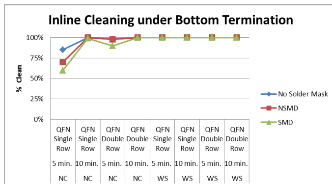
Figure 29: Inline Cleaning under QFN Bottom Termination
