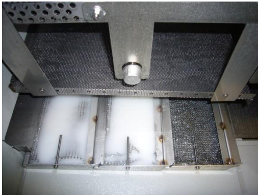
Figure 5: Sluice Box Collection Boxes
