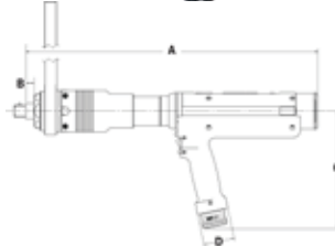
Standard Square Drive Bottom Exit (A) Model
